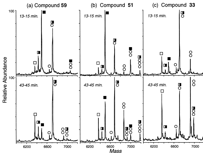
Figure 3. Time course study of zinc ejection from NCp7 by compounds (a) 59 , (b) 51 , and (c) 33 as monitored by ESI-MS. Deconvoluted mass spectra acquired 13–15 min (top) and 43–45 min (bottom) after 150 \mu M of the compound was added to a solution containing 30 \mu M NCp7, 60 \mu M ZnCl 2 , and 10 \mu M ammonium acetate pH 6.9. The square symbol represents the amount of zinc bound to NCp7: a completely filled square (■) designates 2 bound-zinc, a half-filled square (◐) designates 1 bound-zinc, and an open square (□) designates zero bound-zinc (apo-protein). The circle (○) symbol represents covalently-bound compound to NCp7, with the number of circles equal to the number of molecules binding.
