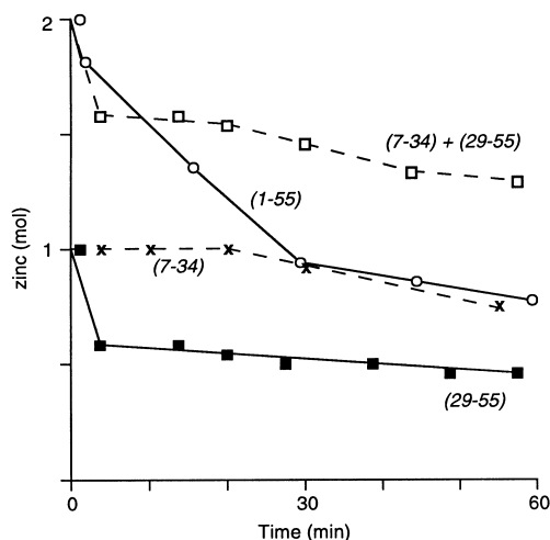
Figure 4. Time course study of total zinc ejection by 2 from zinc-bound peptides derived from the NCp7 amino acid sequence (see Fig. 1) measured by ESI-MS. The following symbols were used to represent the data for the various peptides studied: ■, peptide 29-55; x, peptides 7-34; O, 1-55 (NCp7). Peptides 13-30 and 34-51 showed no ejection of zinc in the presence of 2 over a 1 h period. The open square (□) symbol designate points resulting from the addition of data from peptides 7-34 (x) and 29-55 (■).
