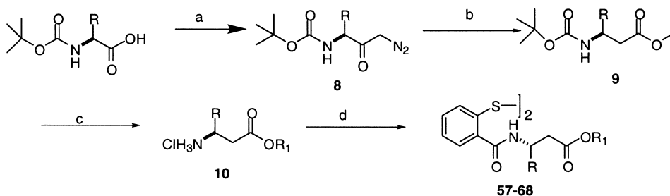
Scheme 2. Reactions conditions: (a) 1 equiv of amino acid, isobutyl chloroformate, triethylamine, –78 °C, 30 min, THF, 1.1 equiv of diazomethane in ether, rt; (b) silver benzoate, triethylamine, methanol; (c) i. R_1 = H ; potassium carbonate, MeOH, H_2O ; ii. 4 N HCl in dioxane, rt, 45 min; (d) bisacid chloride, 6, coupling as in Scheme 1.
