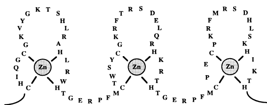
Figure 5. Amino acid sequence of SP1 protein.
