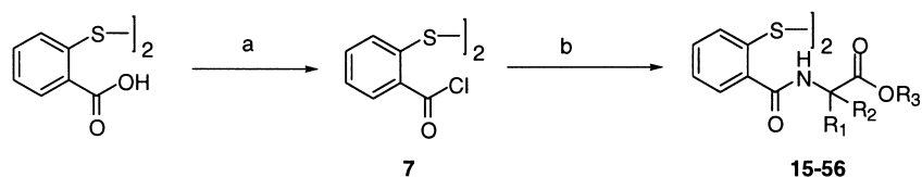
Scheme 1. Reactions conditions: (a) thionyl chloride reflux, overnight; (b) i. 1 equiv of amino acid or its ester, 4.0 equiv of N -methyl- N -(trimethylsilyl)acetamide, N -methylmorpholine dichloromethane, rt, 30 min, followed by addition of bisacid chloride, rt, 4–12 h; or ii. Dichloromethane, triethylamine or N -methylmorpholine, rt, overnight, or iii. 1 equiv of amino acid or its ester, potassium t -butoxide, ethanol, 0 °C, 1 h, followed by addition of bisacid chloride, rt, 4–12 h.
