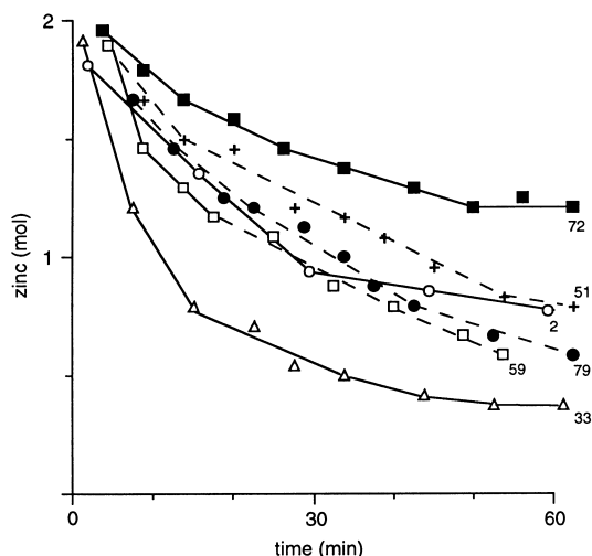
Figure 2. Time course study of total zinc ejection from NCp7 measured by ESI-MS. The absolute abundances (peak intensity) for each protein–zinc species were summed in each mass spectrum acquired at each time point and normalized to the total protein ion signal. For example, all of the ion signals for the NCp7-Zn 1 species were counted together (i.e. [NCp7+Zn]+[NCp7+Zn+drug]+[NCp7+Zn+2drug]+ etc). The following symbols were used to represent the data for the various compounds studied: ■, 72; +, 51; O, 2; ●, 79; □, 59; △, 33.
