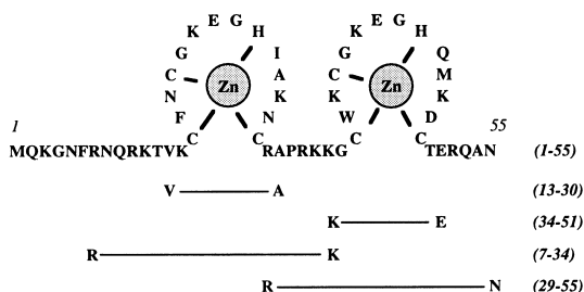
Figure 1. Amino acid sequence of nucleocapsid protein, NCp7, and the peptide fragments used for this study.
