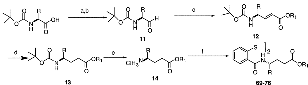
Scheme 3. Reaction conditions: (a) EDCI, HOBT, N -methylmorpholine, HCl·HN(OMe)Me, 0 °C to rt; (b) LAH, 0 °C; (c) Wittig reagent, rt; (d) hydrogenation; (e) i. R = H , 3 N NaOH, rt; ii. 4 N HCl in dioxane, rt; (f) bisacid chloride, 7, coupling as in Scheme 1.
